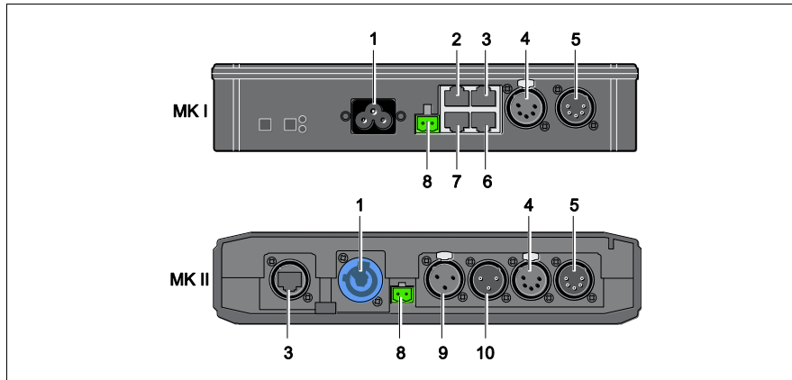
Fig. 2: Connectors and ports of F-1
