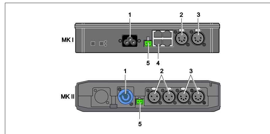
Fig. 7: Connectors and ports of BlackBox R-512
