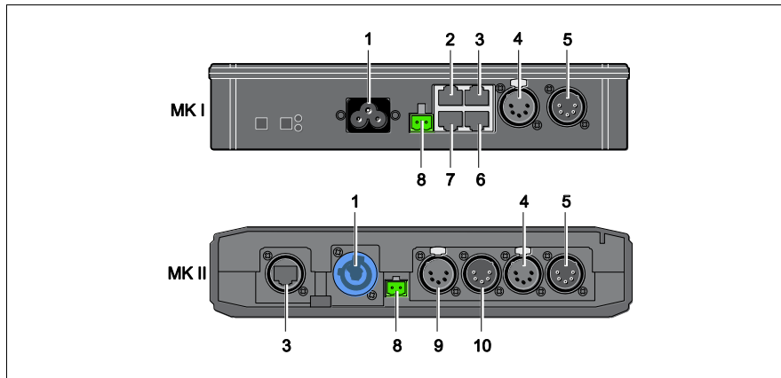
Fig. 8: Connectors and ports of the BlackBox F-2
