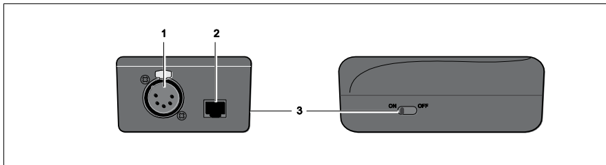
Fig. 14: Micro R-512 Lite, side view
