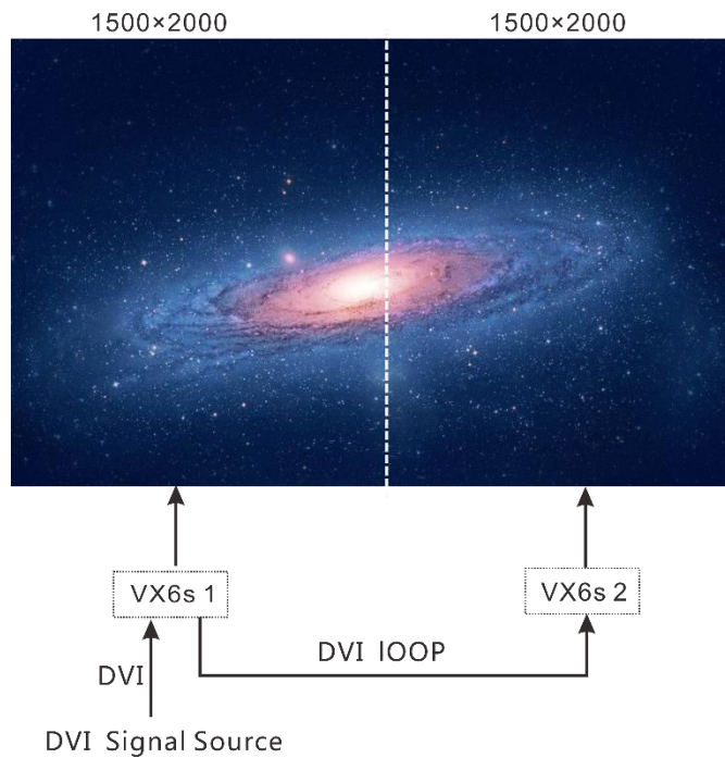
Figure 3-21 Hardware connection for image mosaic
