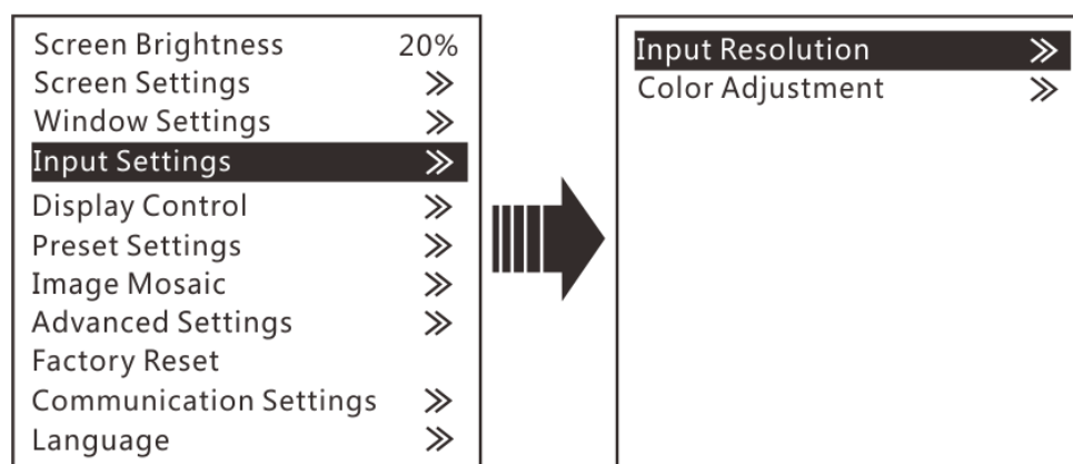
Figure 3-14 Setting input resolution
