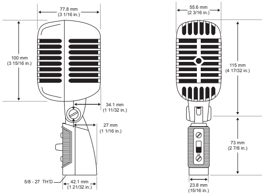
Overall Dimensions
