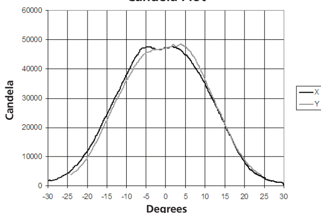
Candela Plot
