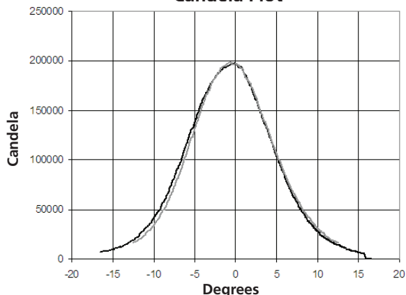
Candela Plot
