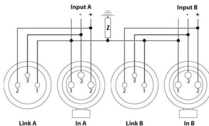
Figure 9: Analog input panel wiring
