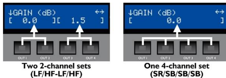
Figure 29: Channel sets
