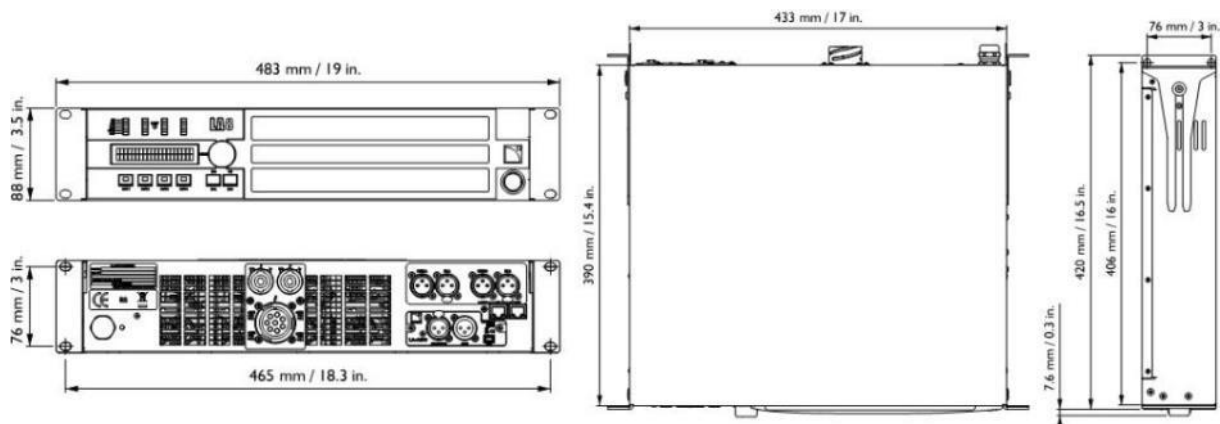
Figure 5: LA8 dimensions
