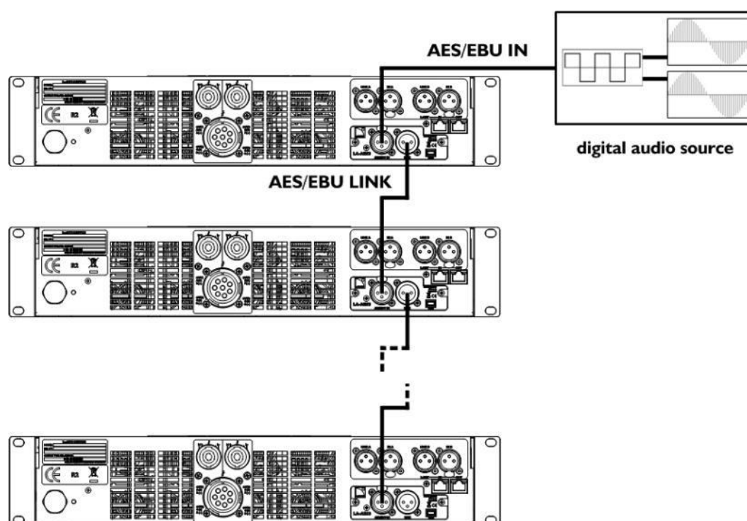
Figure 10: Daisy-chaining digital audio
