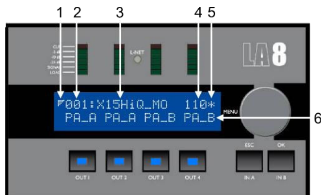
Figure 15: Main screen
