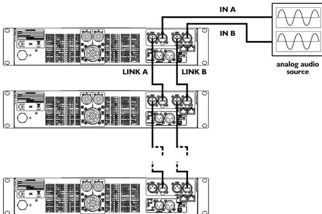
Figure 8: Daisy chaining analog audio
